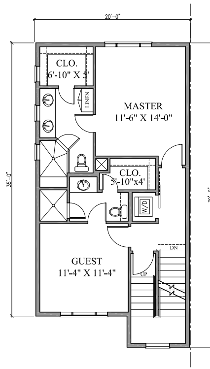
THIRD FLOOR
